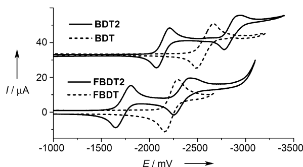
Figure 2. Comparison of cyclic voltammograms in THF/0.1 M Bu 4 N + [PF 6 − ] (1 × 10 −3 mol L −1 ; vs. Fc 0/+ , ν = 100 mV s −1 ).
