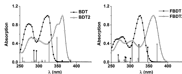
Figure 4. Comparison of UV-Vis spectra in THF. Vertical lines correspond to calculated excitations (TD-DFT, B3LYP/6-31 + G*; see Ref. [15]).
