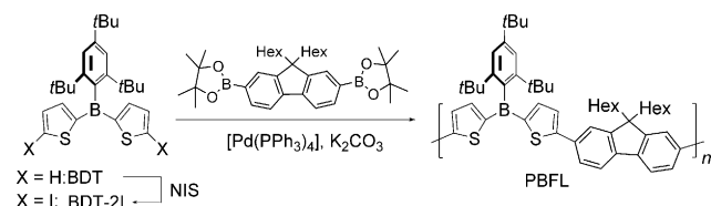
Scheme 2. Synthesis of a conjugated polymer from BDT-2I.
