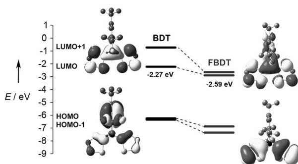
Figure 3. Calculated frontier orbital energy levels and HOMO/LUMO orbital plots of BDT and FBDT (DFT, B3PW91/6-311 + G*; see Ref. [15]).
