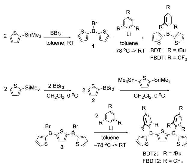
Scheme 1. Synthesis of sterically shielded (oligo)thienylboranes.
