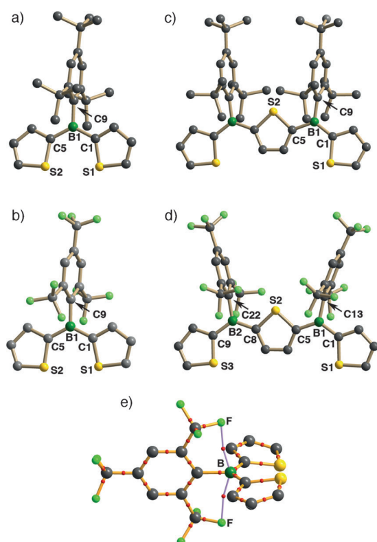
Figure 1. X-ray structure plots of a) BDT, b) FBDT, c) BDT2, d) FBDT2, and e) atoms-in-molecules (AIM) analysis of FBDT, showing B...F bond paths (purple lines) and bond critical points (BCP, red points).
